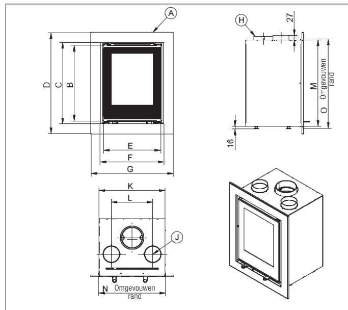
Linear inzethaard XS 500
