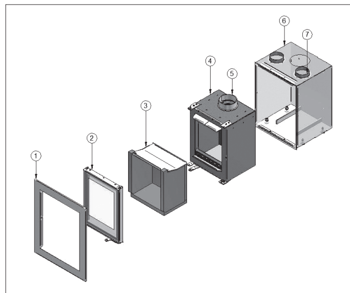
Linear inzethaard XS 500
