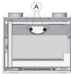
A = Schroeven vanuit de stookkamer losdraaien
