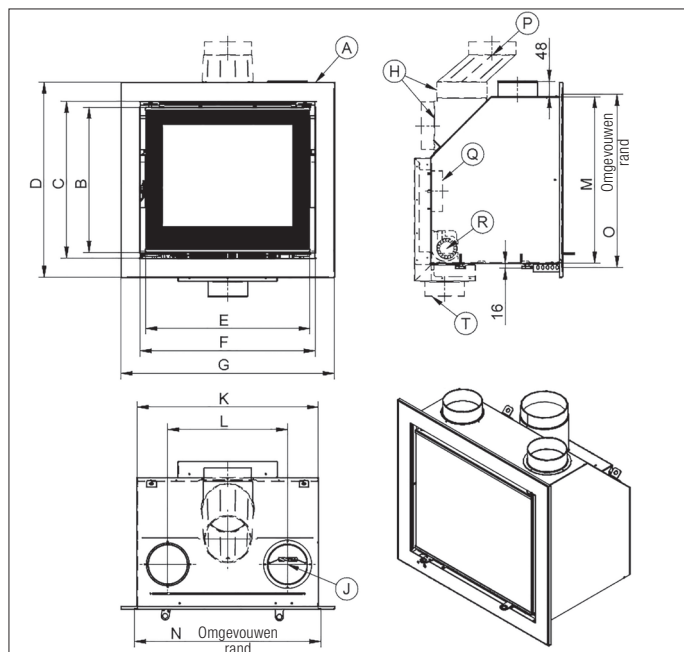
Linear inzethaard 600-900 (S, M, L, XL)
